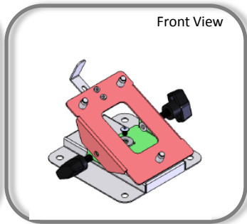
Fixed Height Stand P/N:225758104
